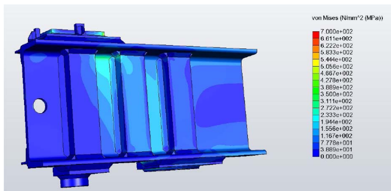
Figure 4: Stress distribution in the reaction beam under the maximum normal load applied. The computed maximum displacement in the beam is 0.33 cm (Finite Element Modelling Simulation)
