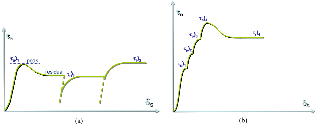
Figure 7: Schematic visualization of direct shear test (a) procedure according to ISRM 1 , (b) proposed step-wise procedure
