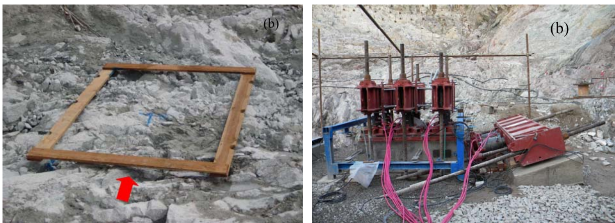
Figure 8: Testing site: (a) rock surface to be sheared, (b) photograph of the shear test apparatus
