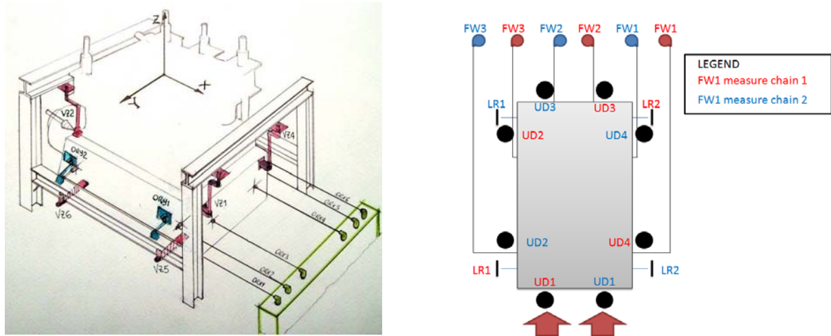
Figure 5: Arrangement of displacement transducers
