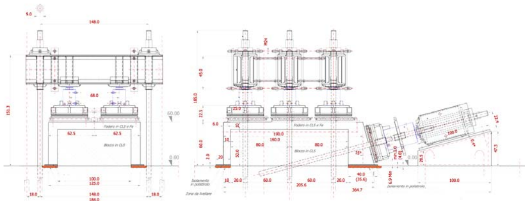
Figure 3: Detailed drawing of the new direct shear apparatus
