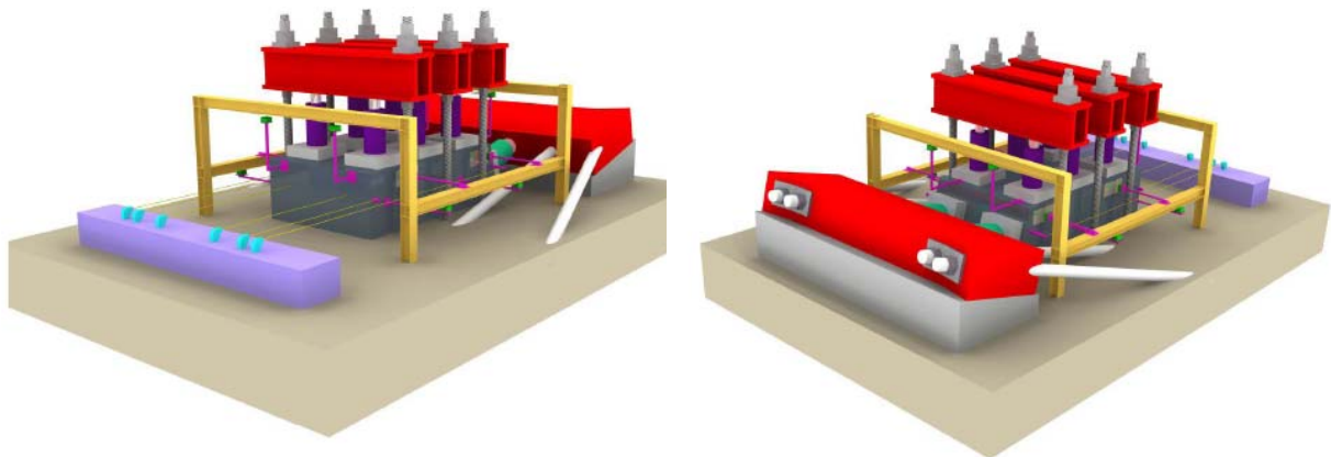
Figure 2: Rendering of the new direct shear apparatus
