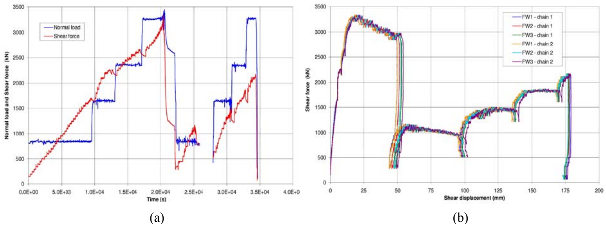
Figure 10: Results of direct shear test on concrete-rock interface with stepwise procedure (a) Normal load N and Shear force S versus time, (b) Shear force S versus Shear displacement \delta_s
