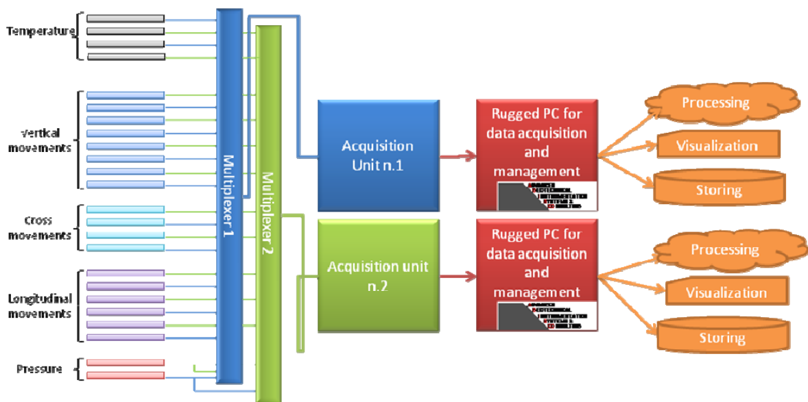
Figure 6: Layout of the data acquisition system
