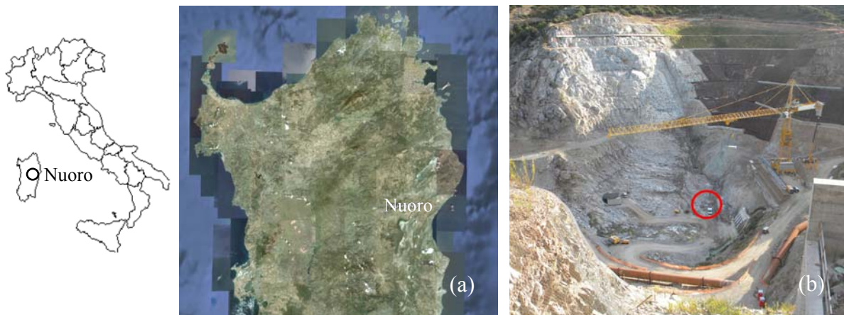
Figure 1: (a) Location of the dam site. (b) View of the foundation surface (right abutment, test site in red circle)
