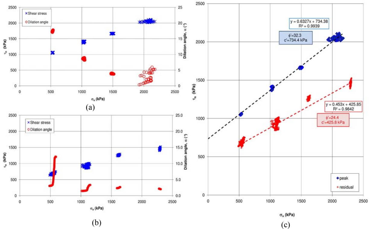
Figure 11: Results of direct shear test on concrete-rock interface with step-wise procedure (a), (b) Plots of shear strength and dilation angle versus normal stress: (a) peak and (b) residual values (c) Plot of shear strength versus normal stress, peak and residual Mohr-Coulomb envelopes.
